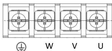
Figure 2.2.2 Fence terminal socket
